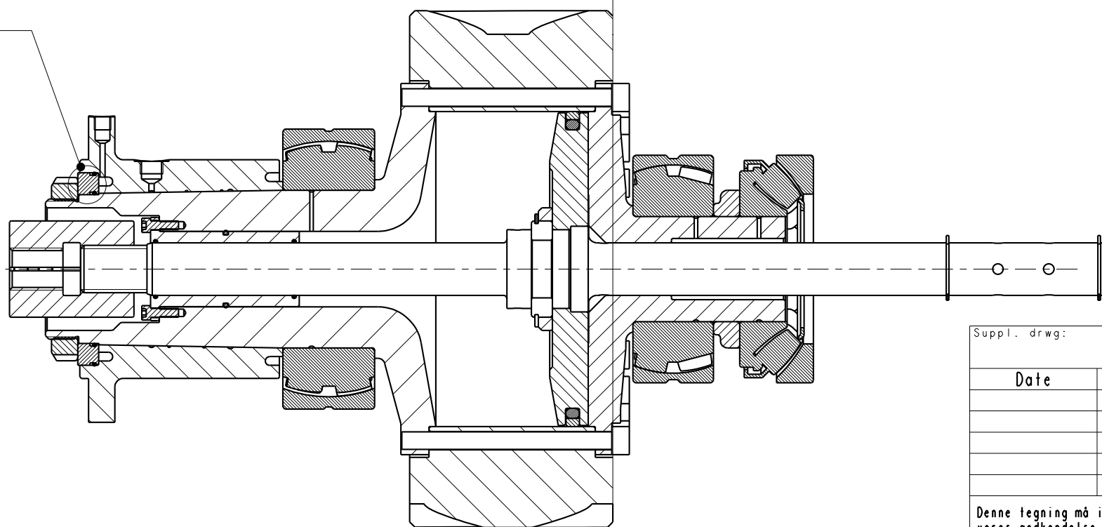
SECTION A-A SCALE 33:100
